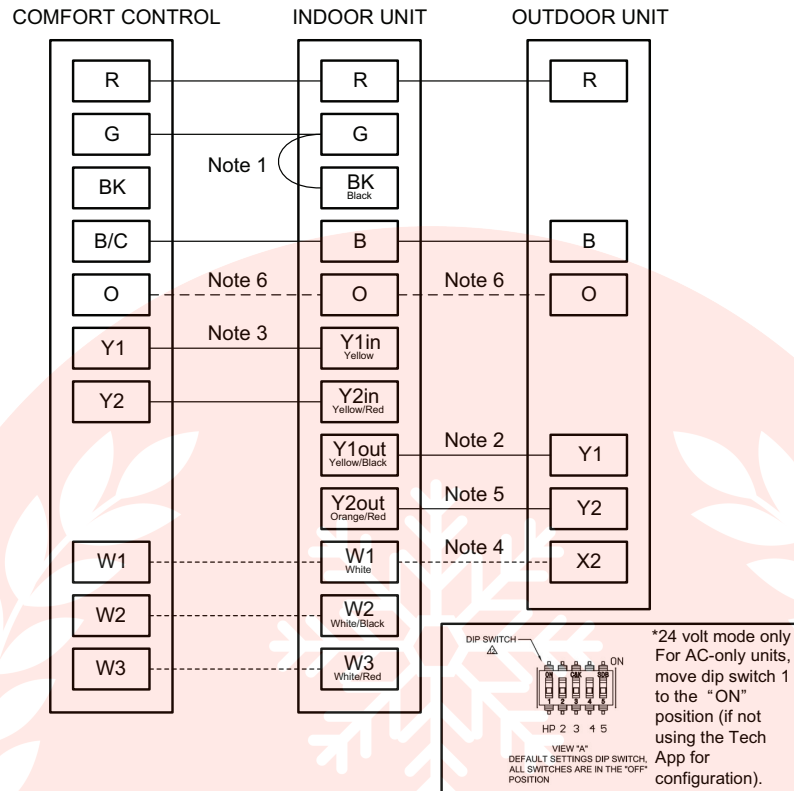
Figure 4. 24 volt low voltage wiring - 24v multi- stage system, AC or HP
