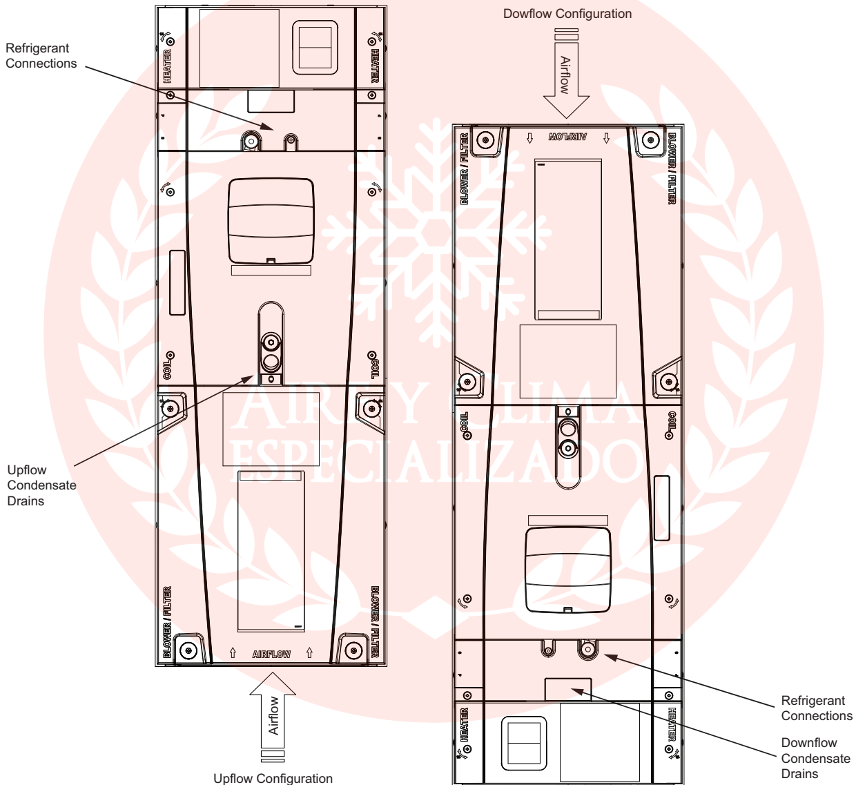
Figure 6. Upflow and downflow configuration
