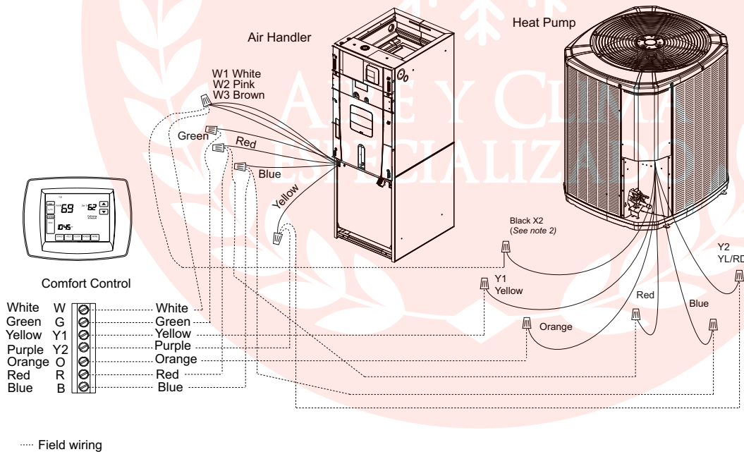
Figure 6. Air handler connection diagram – 2 stage HP
