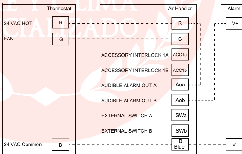
24VAC Audible Alarm, typical
