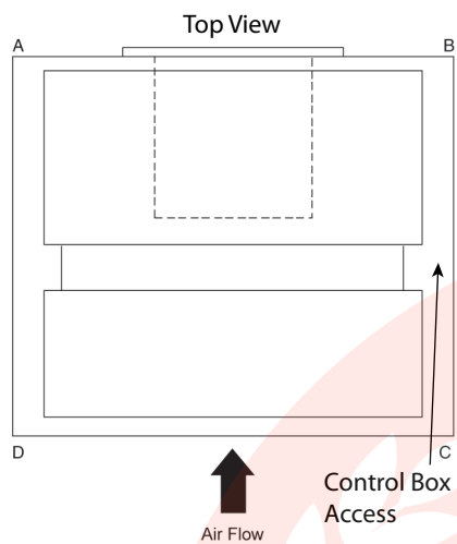
Figure 54. Horizontal — TWE150, 180, 240, 300
