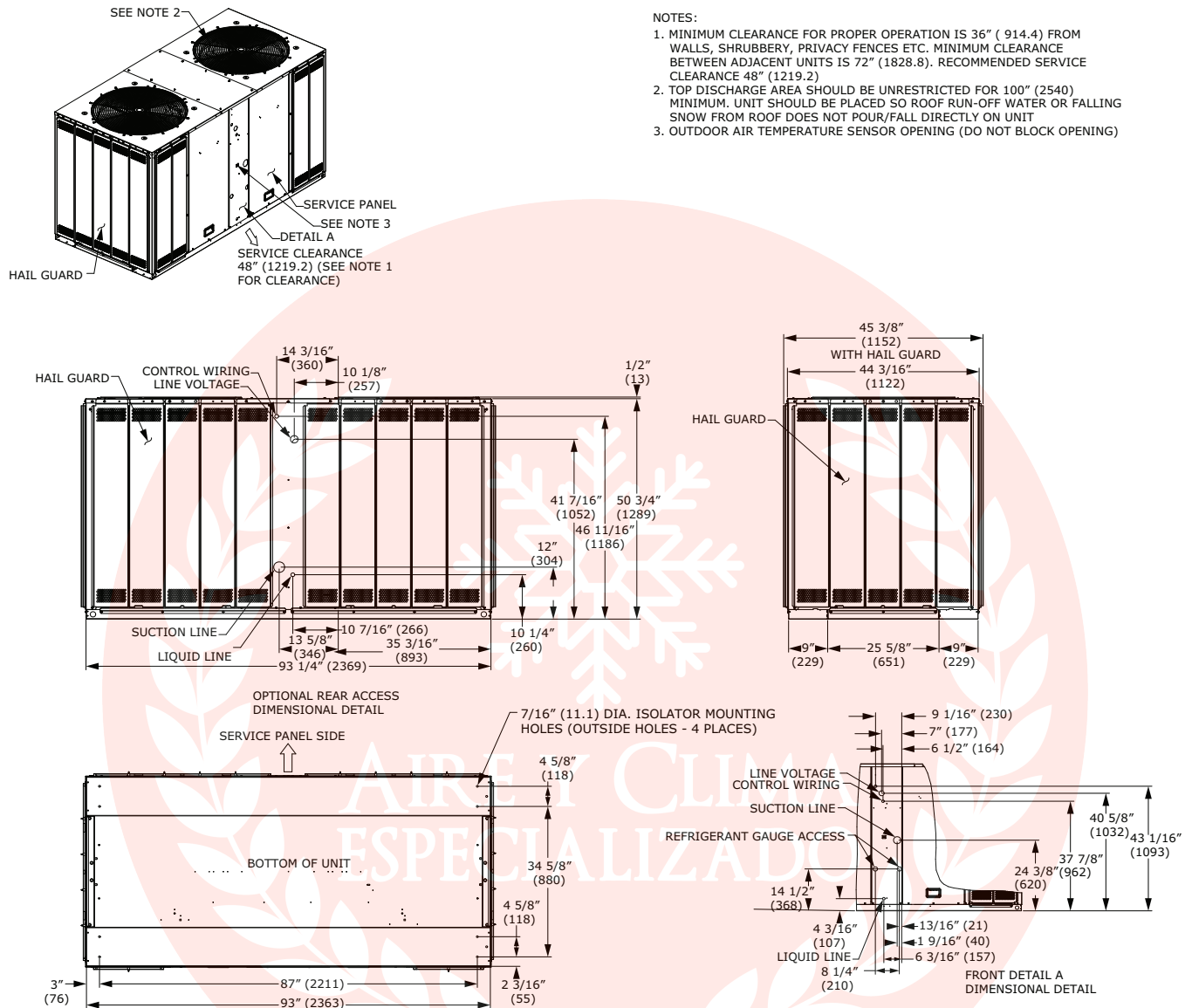
Figure 31. 25 ton condensing, manifolded compressor – in (mm)
